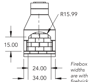
Stone Age Brick Oven weight: 1,600 lbs. Cooking surface area: 670 sq. in.
