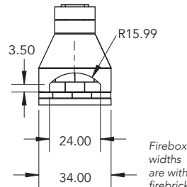
Vecchio Pizza Oven weight: 1,100 lbs. Cooking surface area: 670 sq. in.
