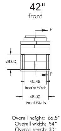
Zero-Clearance Rated Fireplace when installed with Full Fire Brick
