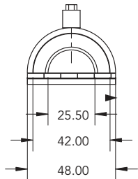
Amerigo Pizza Oven weight: 1,650 lbs. Cooking surface area: 1500 sq. in.
