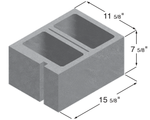
12 x 8 x 16 Hollow Corner Sash
