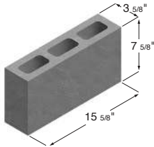
4 x 8 x 16 Hollow Pier
