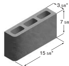
4 x 8 x 16 Hollow Single Bullnose Corner
