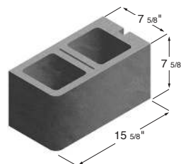
8 x 8 x 16 Hollow Single Bullnose Corner Sash
