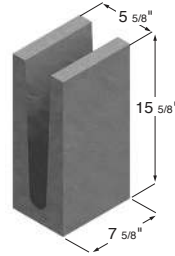
6 x 16 x 8 Bond Beam Lintel
