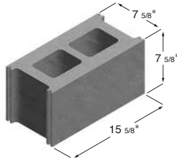
8 x 8 x 16 Hollow 3 Hour Fire Rated
