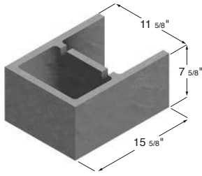
12 x 8 x 16 A-Shaped Block
