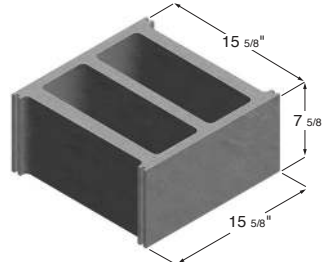
16 x 8 x 16 Hollow Stretcher
