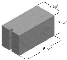
8 x 8 x 16 Solid Corner Sash
