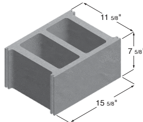
12 x 8 x 16 Hollow Stretcher
