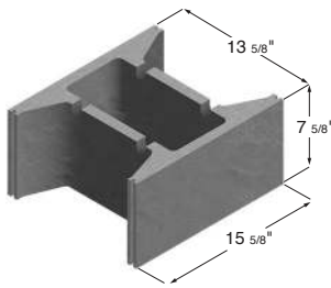
14 x 8 x 16 Open End
