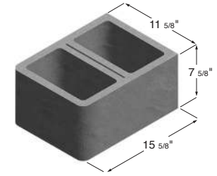
12 x 8 x 16 Hollow Double Bullnose Corner
