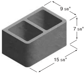
10 x 8 x 16 Hollow Single Bullnose Pier
