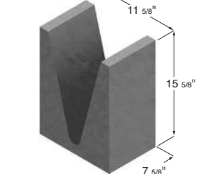
12 x 16 x 8 Bond Beam Lintel
