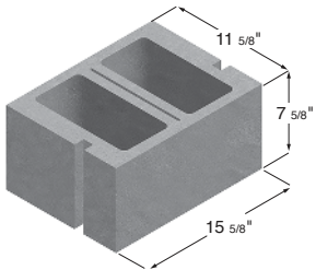
12 x 8 x 16 Hollow Double Sash
