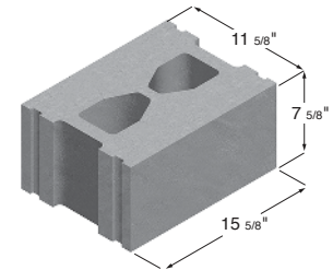
12 x 8 x 16 Semi-Solid Stretcher
