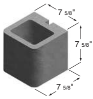
8 x 8 x 8 Hollow Double Bullnose Corner Sash
