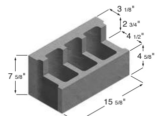
8 x 8 x 16 Hollow Header
