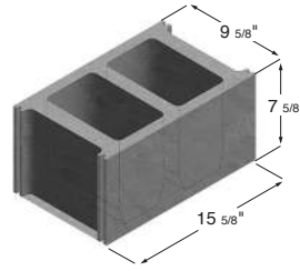
10 x 8 x 16 Hollow Cap 2 Core
