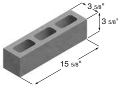
4 x 4 x 16 Hollow Pier
