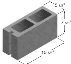
6 x 8 x 16 Hollow Corner Sash
