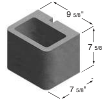
10 x 8 x 8 Hollow Double Bullnose Corner Sash
