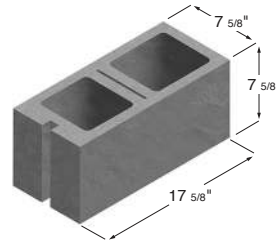
8 x 8 x 18 Hollow Corner Sash
