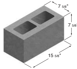
8 x 8 x 16 Semi-Solid Pier
