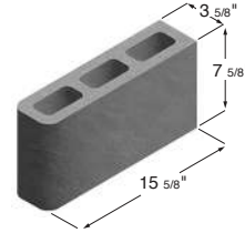
4 x 8 x 16 Hollow Double Bullnose Corner
