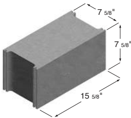
8 x 8 x 16 Solid Stretcher
