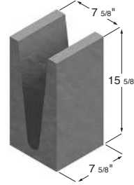
8 x 16 x 8 Bond Beam Lintel
