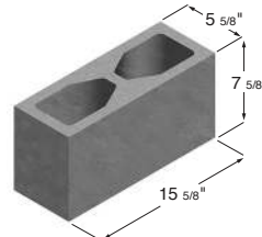
6 x 8 x 16 Hollow Pier
