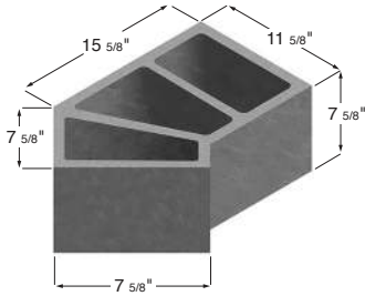
12 x 8 x 21 45 Degree Angle
