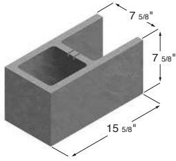
8 x 8 x 16 A-Shaped Block
