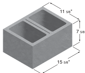
12 x 8 x 16 Hollow Pier
