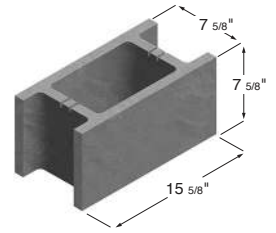
8 x 8 x 16 Open End
