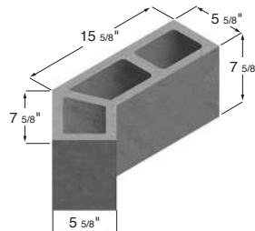
6 x 8 x 21 45 Degree Angle
