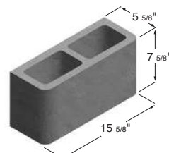
6 x 8 x 16 Hollow Single Bullnose Pier
