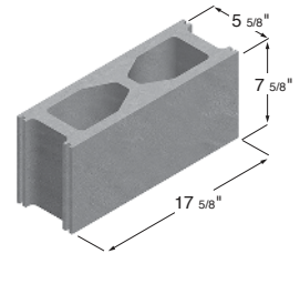
6 x 8 x 18 Hollow Stretcher
