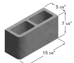
6 x 8 x 16 Hollow Single Bullnose Corner
