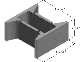
16 x 8 x 16 Open End
