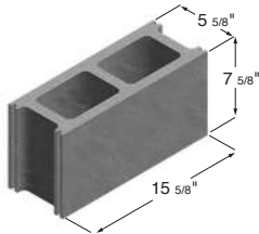
6 x 8 x 16 Hollow Stretcher
