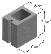
6 x 8 x 8 Hollow Corner Sash
