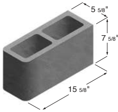
6 x 8 x 16 Hollow Double Bullnose Corner
