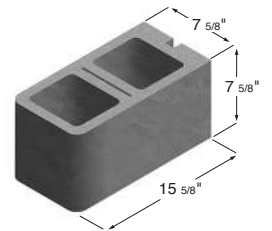
8 x 8 x 16 Hollow Double Bullnose Corner Sash
