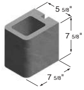
6 x 8 x 8 Hollow Double Bullnose Corner Sash
