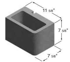
12 x 8 x 8 Hollow Single Bullnose Corner Sash
