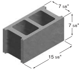
8 x 8 x 16 Hollow Stretcher
