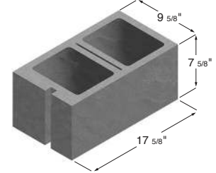
10 x 8 x 18 Hollow Corner Sash
