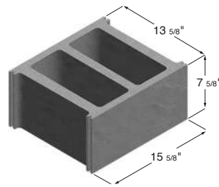
14 x 8 x 16 Hollow Stretcher
