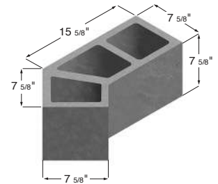
8 x 8 x 21 45 Degree Angle
