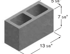
6 x 8 x 14 Hollow Pier
