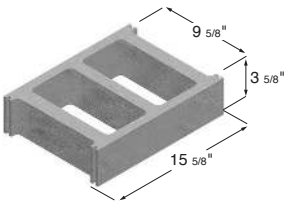
10 x 4 x 16 Hollow Stretcher
